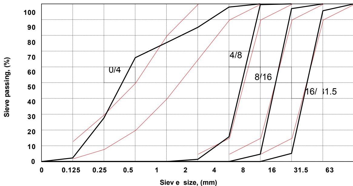
Figure 4. Grading curves of natural aggregate.
