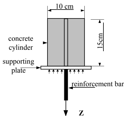
Figure 7. Testing of bond between concrete and reinforcement.
