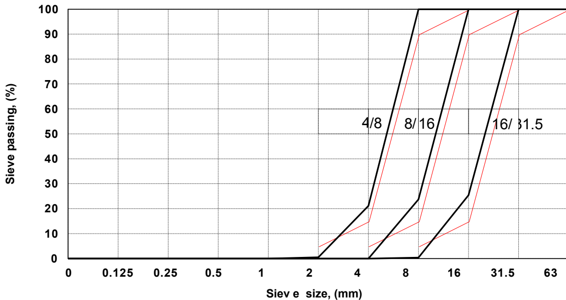
Figure 5. Grading curves of recycled concrete aggregate.
